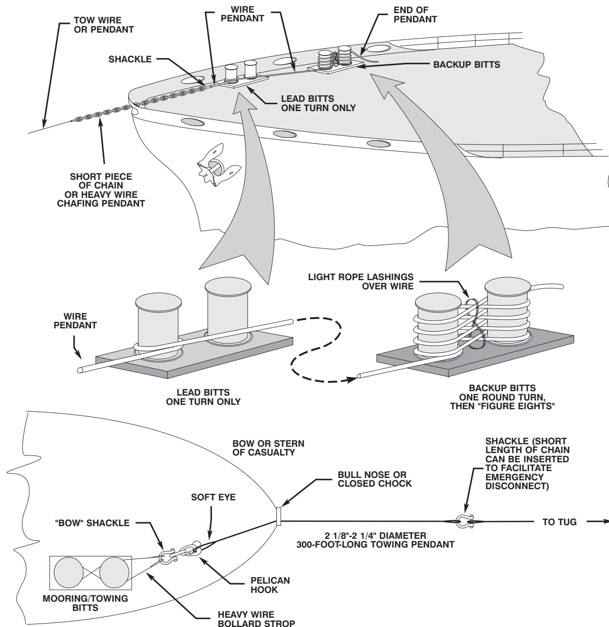
Figure 19-6. Emergency Towing Connections Suitable for Rigging on Disabled Burning Casualties.
