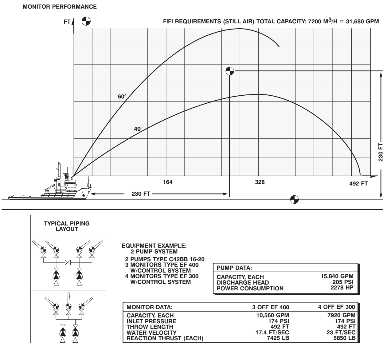
Figure 19-13. FiFi-2 Requirements for Firefighting Systems.
