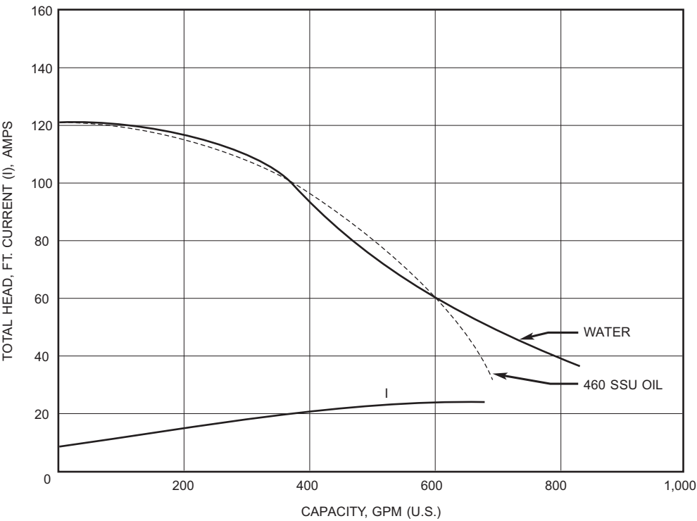
Figure H-6. U.S. Navy 4-Inch Electric Submersible Pump Performance With Impeller No. 2.
