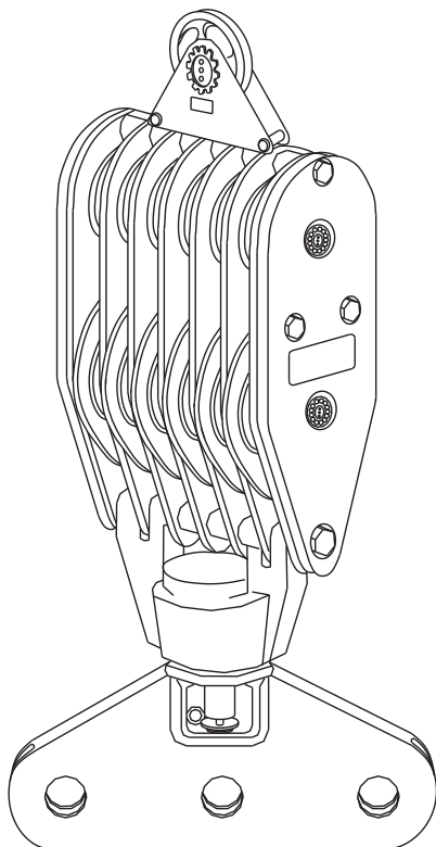
30" AND 24" 250-TON TWELVE-SHEAVE TANDEM SHEAVE BLOCK WITH EQUALIZER AND LOCKING HANGER
