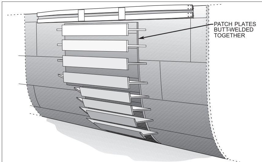
Figure 10-24. Built-Up Steel Patch.
