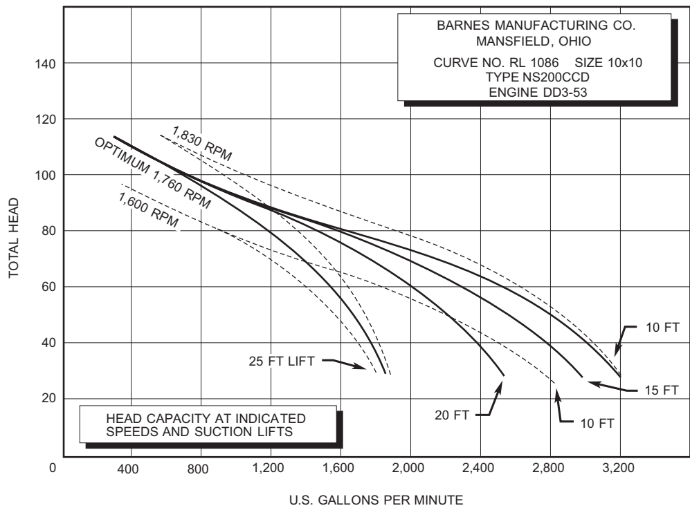
Figure H-3. Performance Curve, 10-Inch Diesel Pump.
