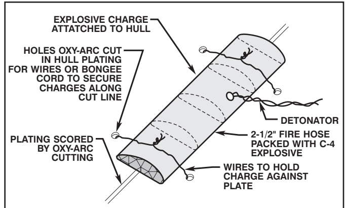
Figure 14-25. Hose-Type Cutting Charge.
