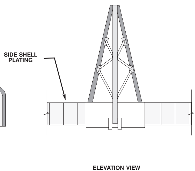
Figure 7-14. Braced-Girder Headframe.
