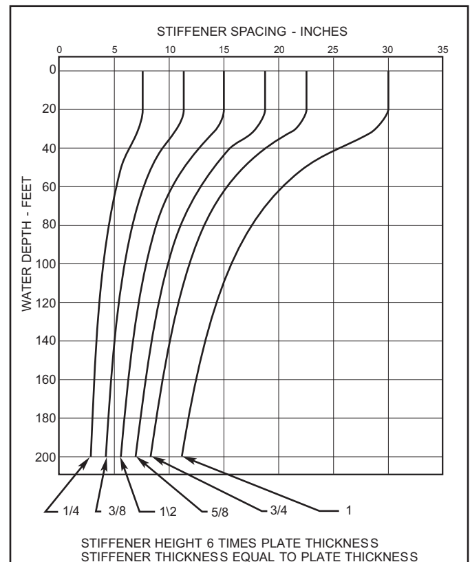
Figure 10-5. Aluminum Patch Stiffener Spacing. Patch Reinforced with Concrete.
