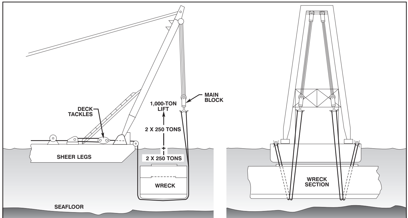
Figure 13-24. Typical Working Arrangements on Salvage Sheer Legs.
