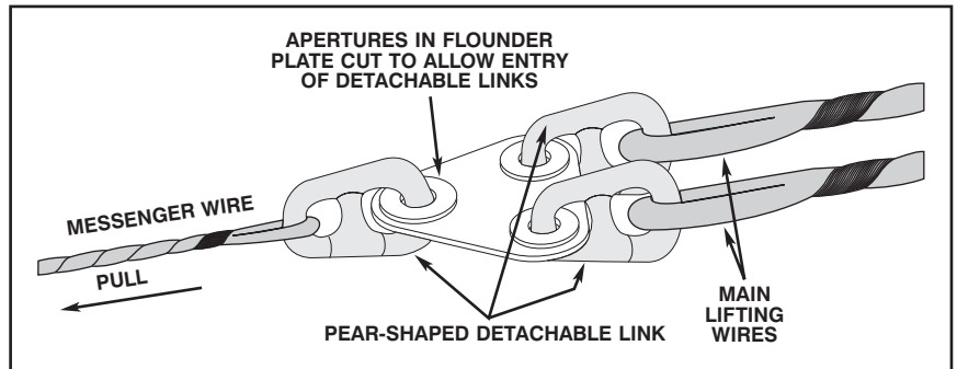
Figure 12-27A. Wire Rigged to Flounder Plate for Passing.
