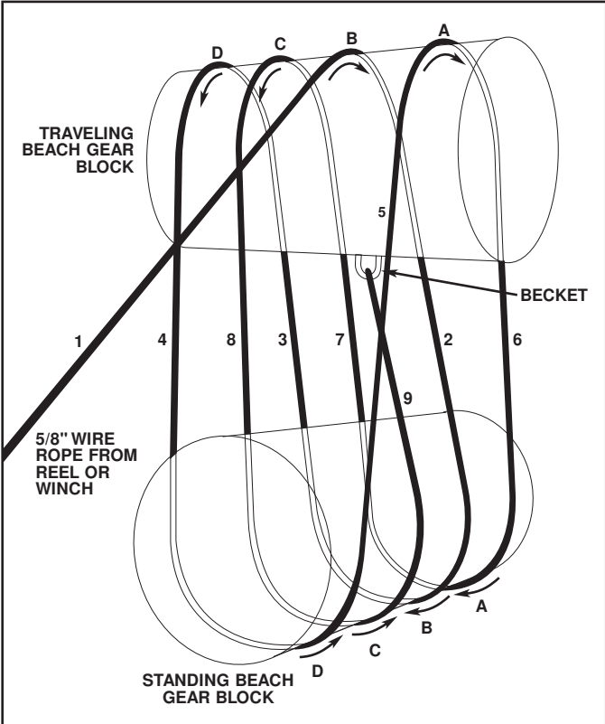
Figure 8-13. Center-to-Center Reeving.
