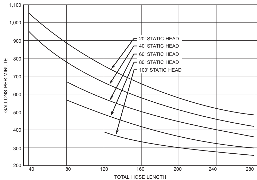
Figure H-13. CCN-150 Flow Rates - Warm #6 Fuel, 6" Hose.
