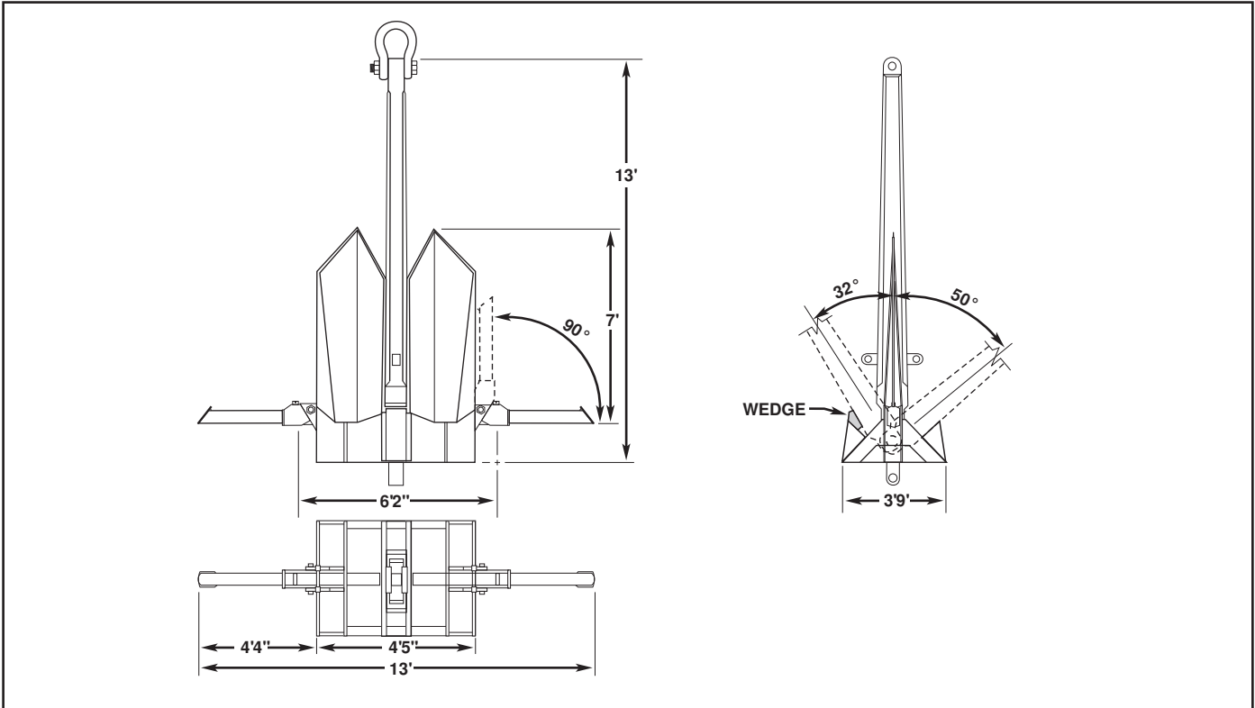
Figure F-10. 6,000-Pound NAVMOOR Anchor Dimensions.
