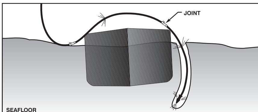
Figure 12-25A. Tunneling Lance Operations.
