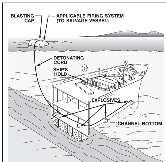
Figure 14-29. Charge Placement for Wreck Settling.
