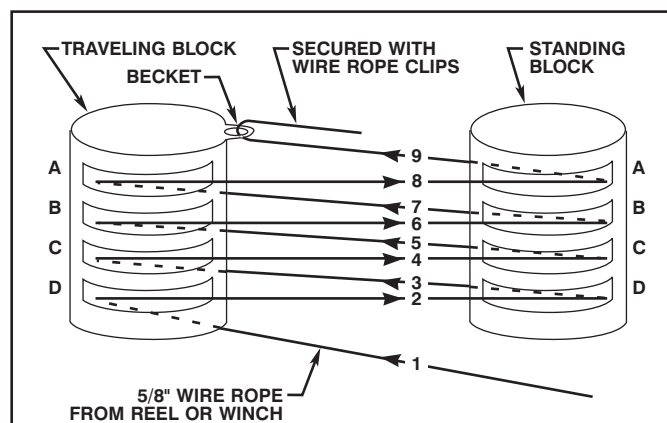
Figure 12-5. Navy Standard Beach Gear Blocks - Round-Robin Reeving.
