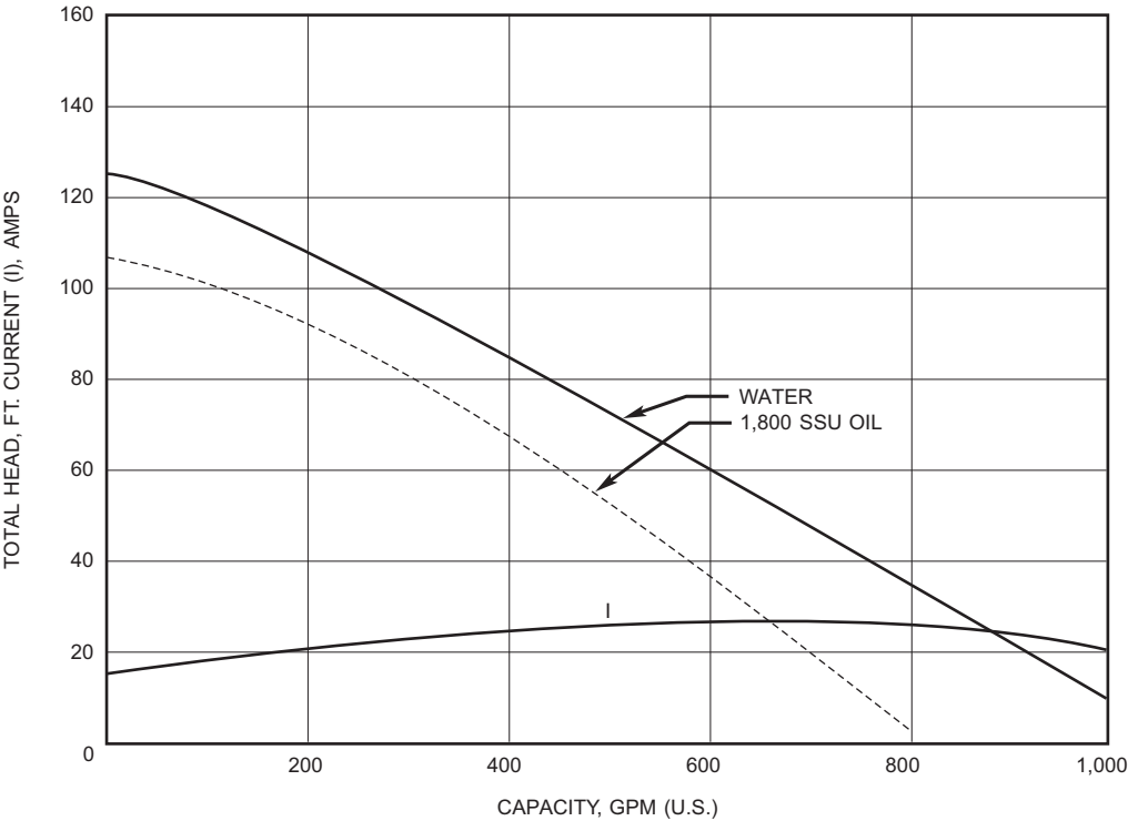
Figure H-7. U.S. Navy 4-Inch Electric Submersible Pump Performance With Impeller No. 3
