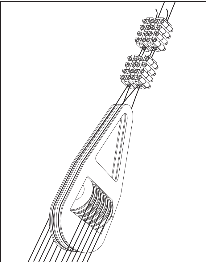
Figure 12-11. Combined Traveling Block and Deadeye.
