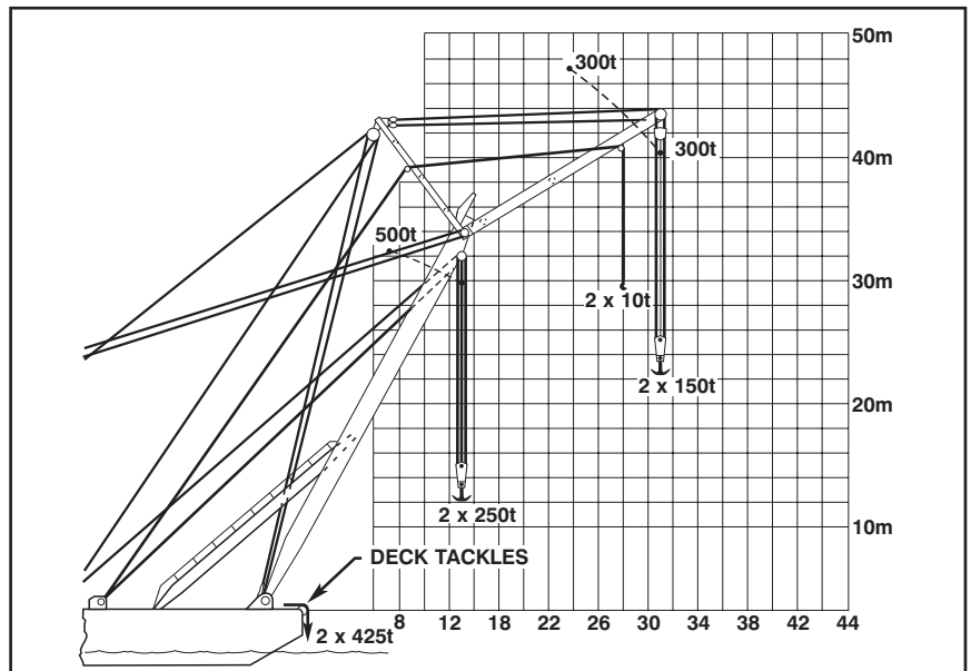
Figure 13-23. Typical Outreach and Lift Diagram for Salvage Sheer Legs.
