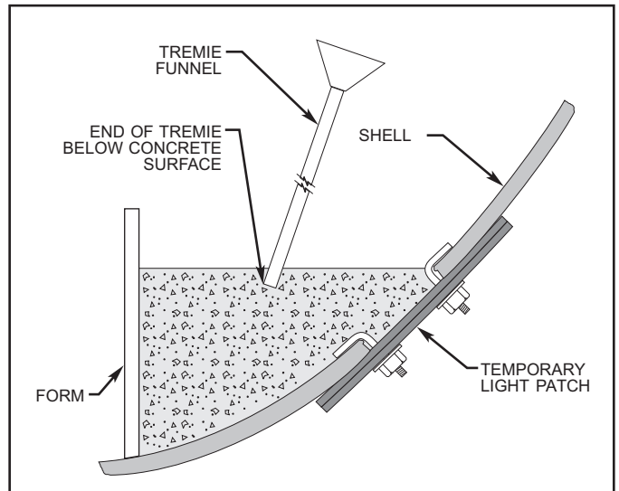
Figure 10-27. Placing Concrete with a Tremie.
