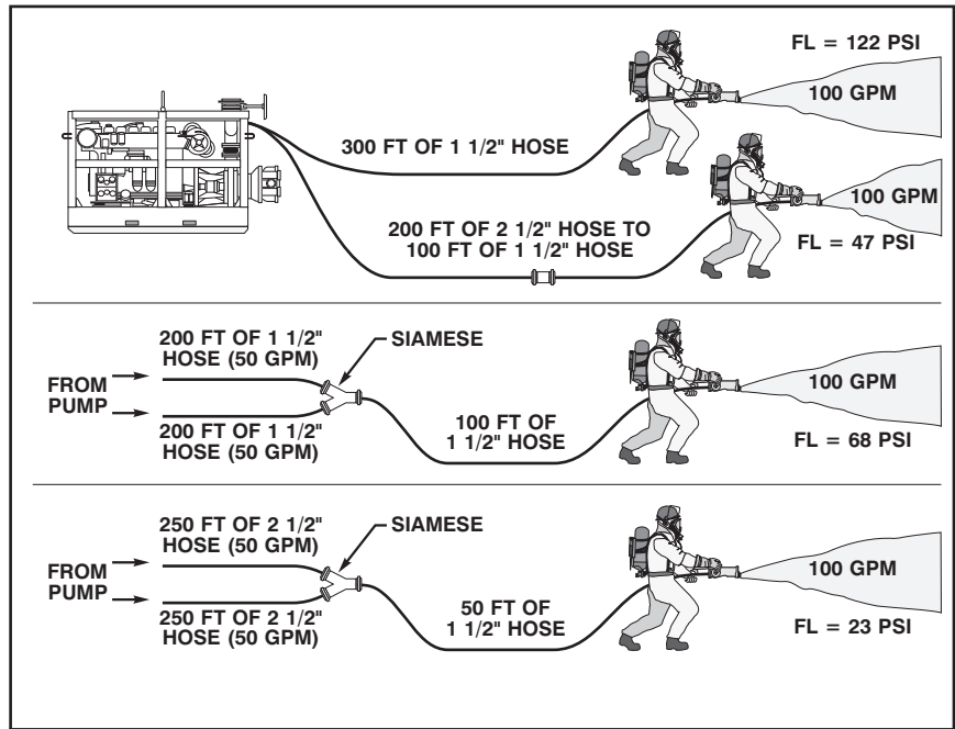
Figure 16-6A. Minimizing Friction Loss.
