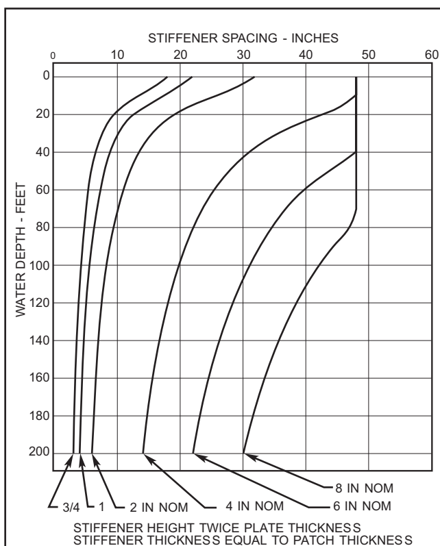
Figure 10-7. Wooden Patch Stiffener Spacing. Patch Not Reinforced with Concrete.
