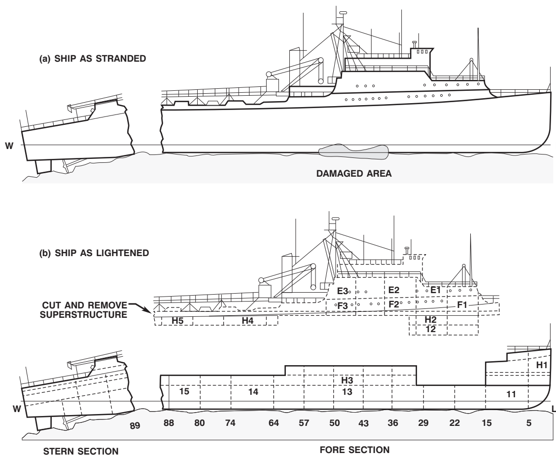
Figure 14-12. Surface Cutting Plan to Lighten a Wreck.
