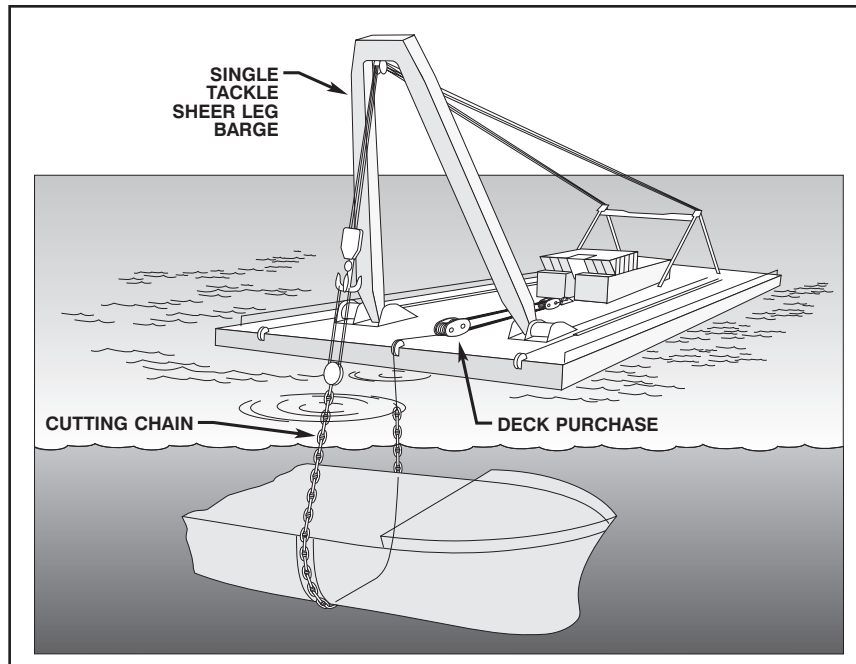
Figure 14-15. Improvised Chain Cutting System with A-Frame and Deck Tackle.
