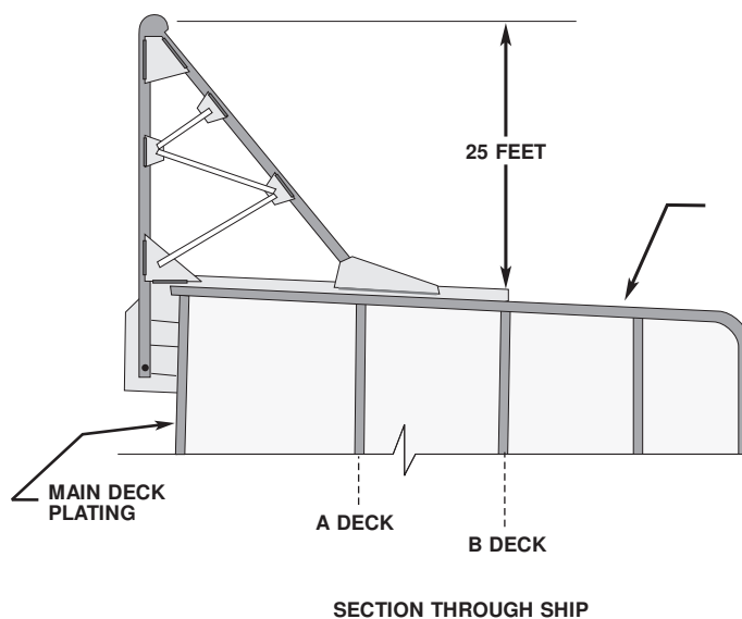
Figure 7-14. Braced-Girder Headframe.
