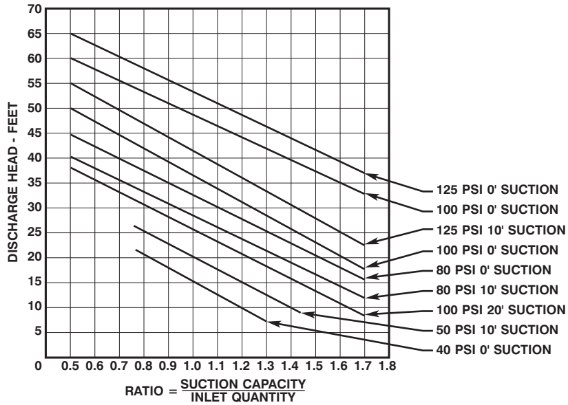
Figure 11-4. Eductor Performance Curve.
