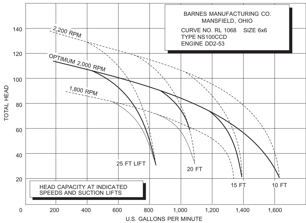
Figure H-2. Performance Curve, 6-Inch Diesel Pump.
