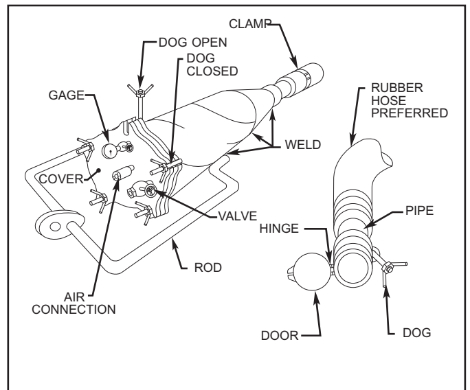
Figure 10-28. Cement Gun.
