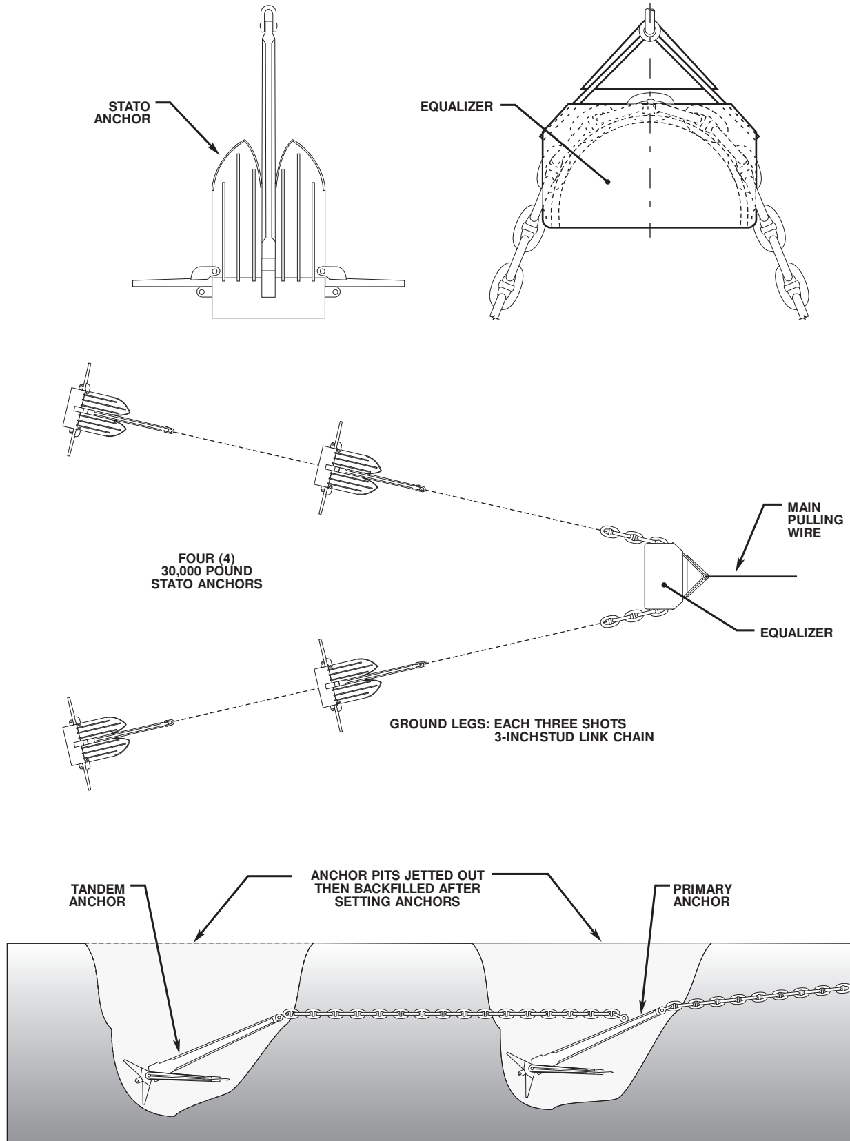
Figure 7-24. Yoked Anchor Placement Pattern.
