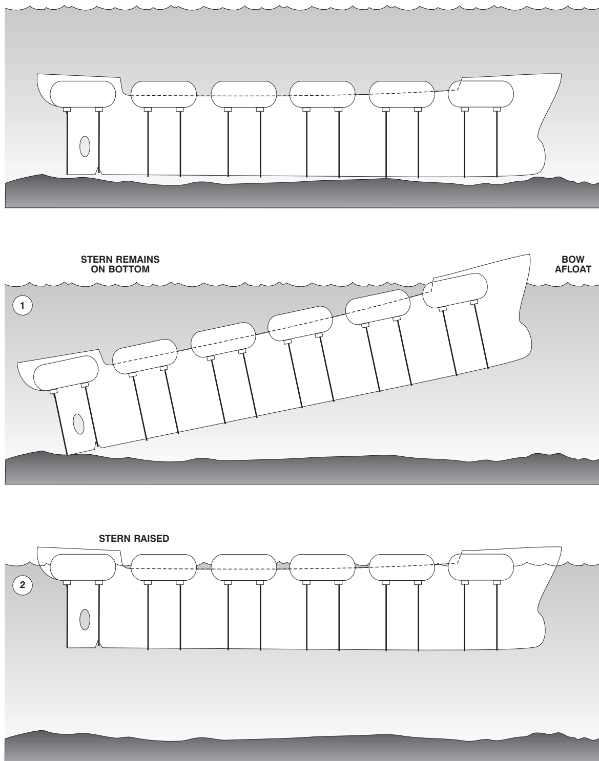
Figure 13-12. Pontoons Raising a Ship Sunk in Shallow Water.
