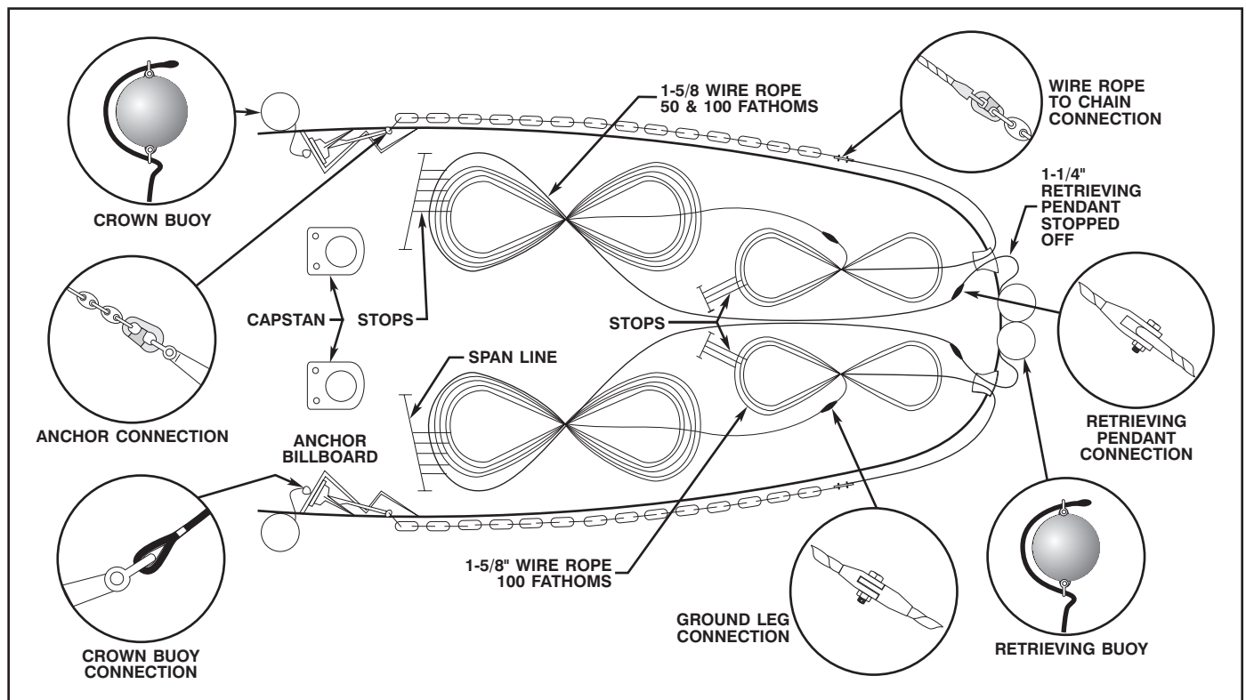
Figure 9-9. Arrangement for Laying the Ground Leg from Seaward Toward the Casualty.
