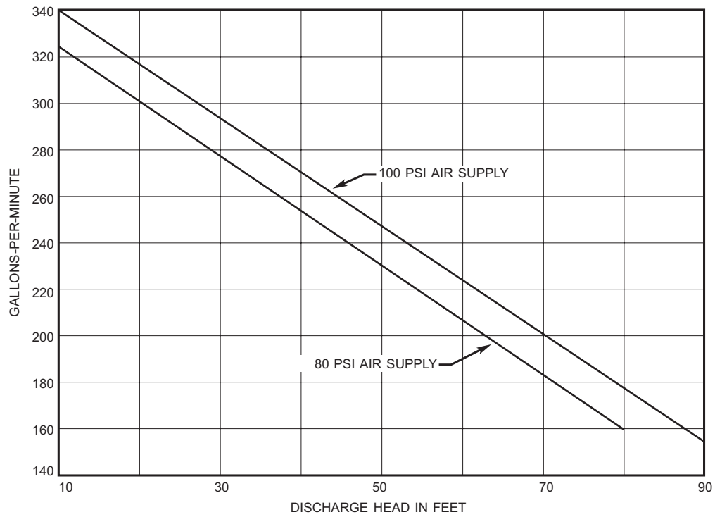
Figure H-4. 2 1/2-Inch Pneumatic Submersible Pump Performance Curves.
