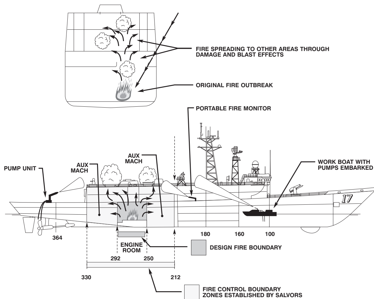
Figure 18-1. Design- and Salvor-Imposed Fire Zone Boundaries.
