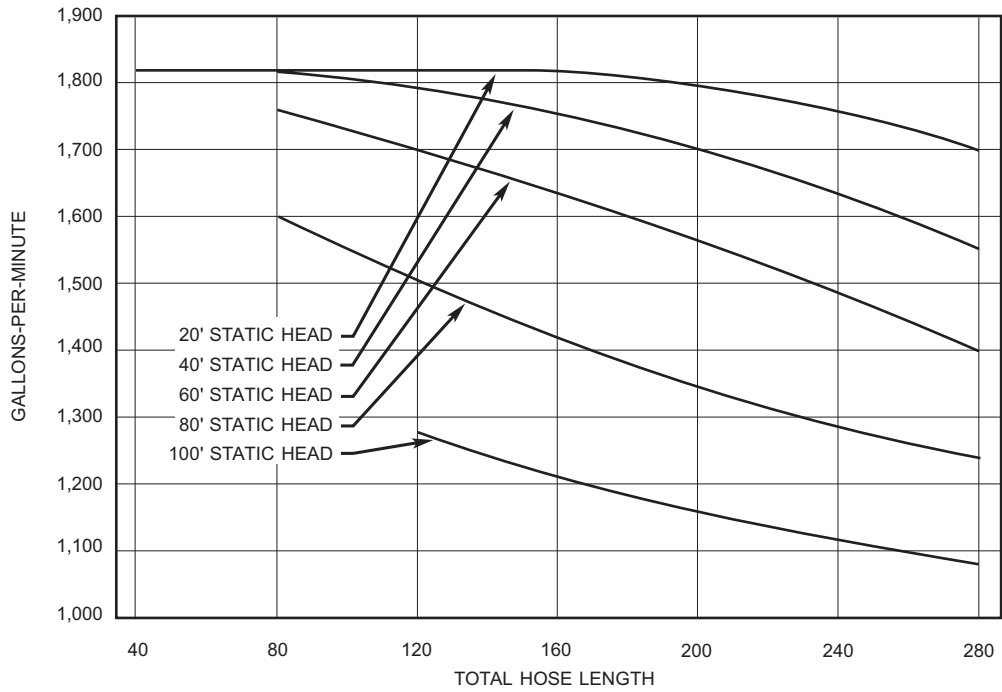
Figure H-11. CCN-150 Flow Rates - Water, 6" Hose.
