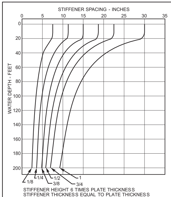
Figure 10-8. Aluminum Patch Stiffener Spacing. Patch Not Reinforced with Concrete.
