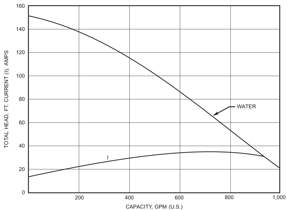
Figure H-5. U.S. Navy 4-Inch Electric Submersible Pump Performance With Impeller No. 1.
