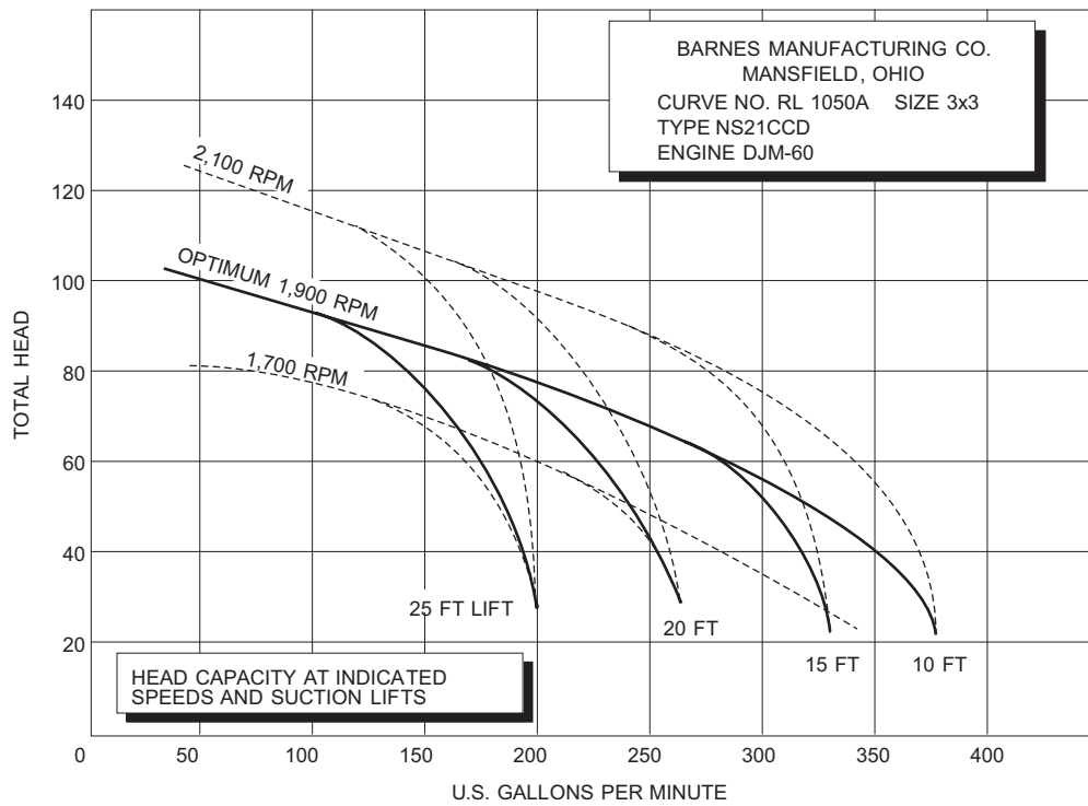
Figure H-1. Performance Curve, 3-Inch Diesel Pump.
