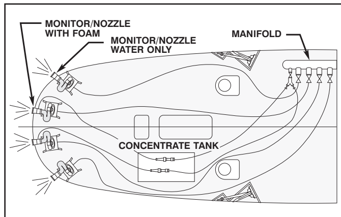
Figure 17-6. Offship Manifold and Portable Equipment.
