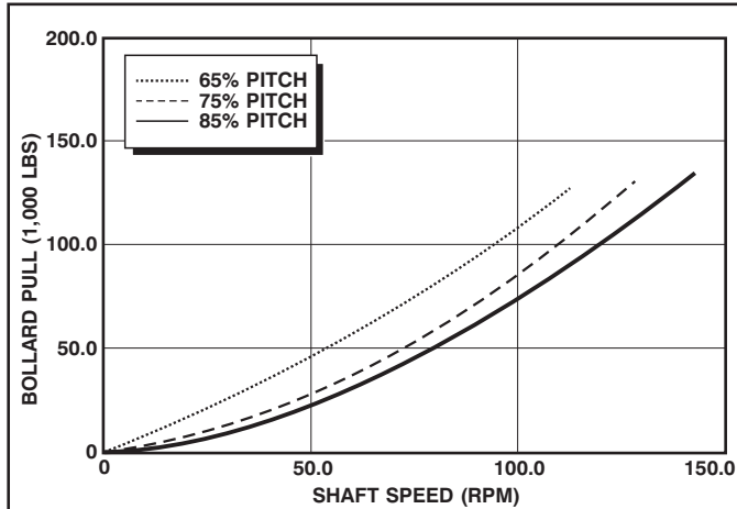
Figure G-1. Variation of Bollard Pull with Shaft Speed and Propeller Pitch for ARS-50 Class Ships.
