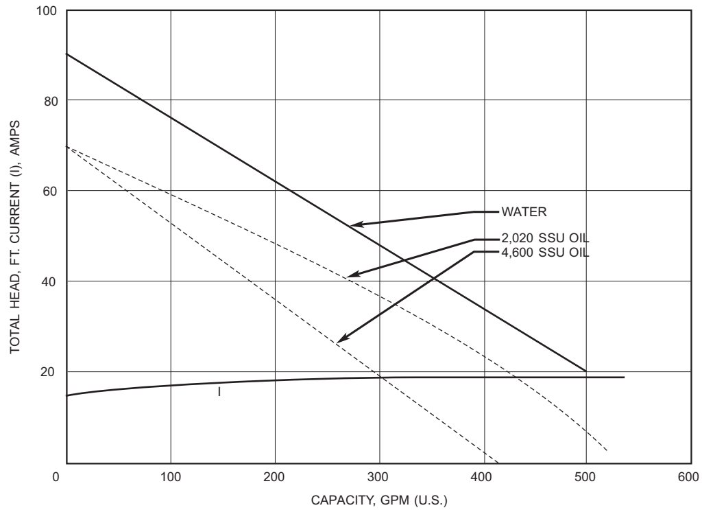
Figure H-8. U.S. Navy 4-Inch Electric Submersible Pump Performance With Impeller No. 4.
