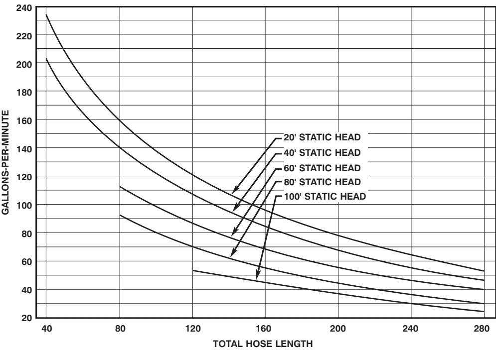
Figure H-15. CCN-150 Flow Rates - Cold #6 Fuel, 6" Hose.
