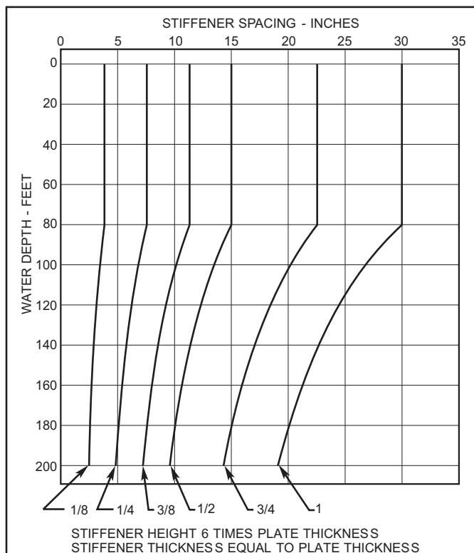
Figure 10-6. Steel Patch Stiffener Spacing. Patch Reinforced with Concrete.
