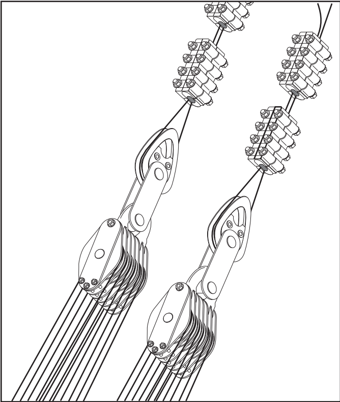
Figure 12-10. Lift Wires Made Up with Bullivant Clamps.
