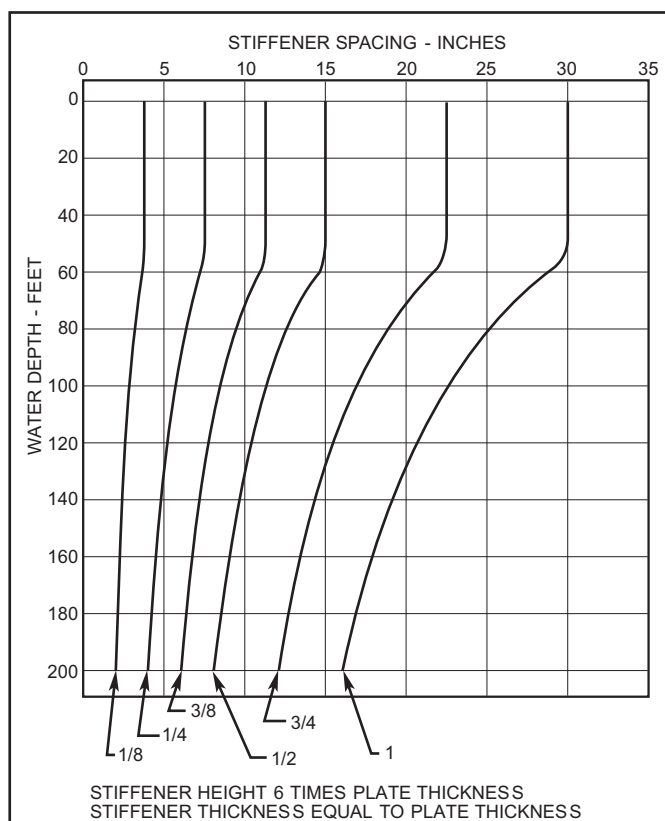
Figure 10-9. Steel Patch Stiffener Spacing. Patch Not Reinforced with Concrete.
