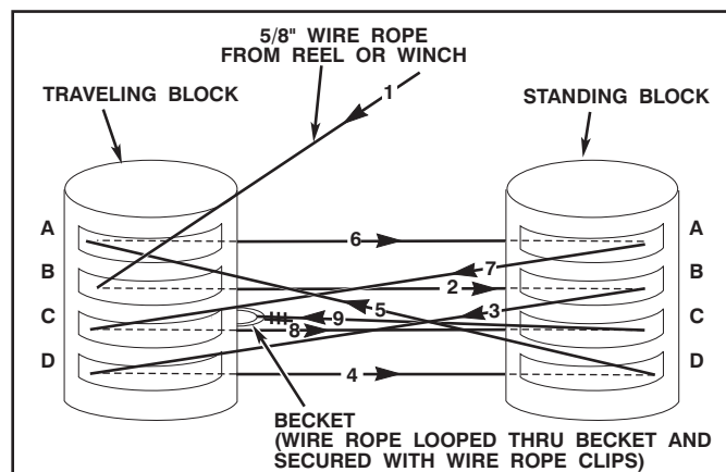
Figure 12-4. Navy Standard Beach Gear Blocks - Center to Center Reeving.
