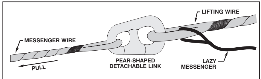
Figure 12-26. Wire Messengers Connected with Detachable Link.
