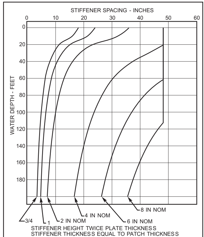
Figure 10-4. Wooden Patch Stiffener Spacing. Patch Reinforced with Concrete.
