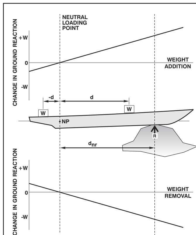
Figure 6-4. Effects of Weight Changes on Ground Reaction.
