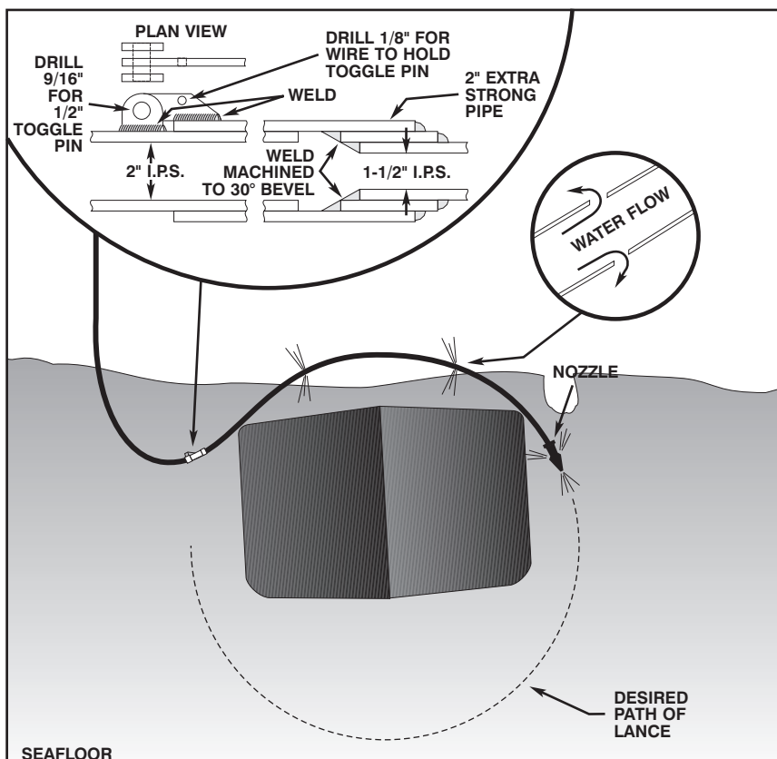
Figure 12-24. Tunneling Lance Operations.
