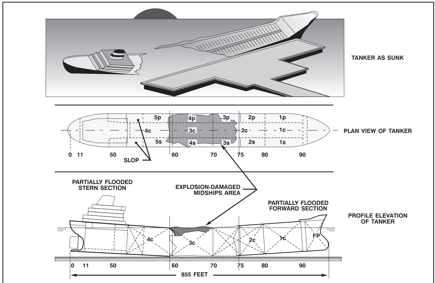
Figure 14-4. Tanker Wreck as Surveyed.
