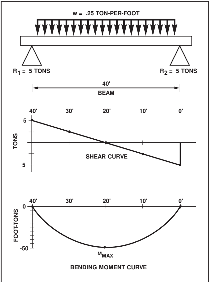
Figure 5-6. Bending Moment and Shear Curves for Example 5-3.
