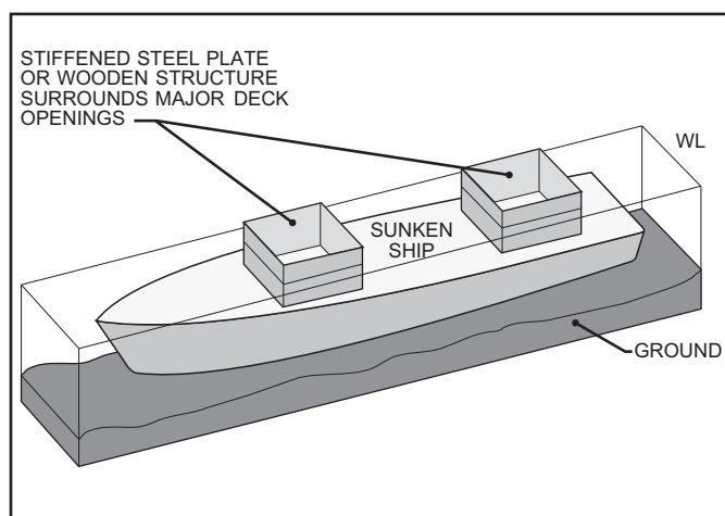
Figure 10-39. Partial Cofferdams.
