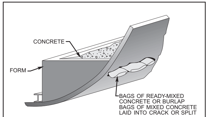
Figure 10-29. Concrete Crack or Split Repair.
