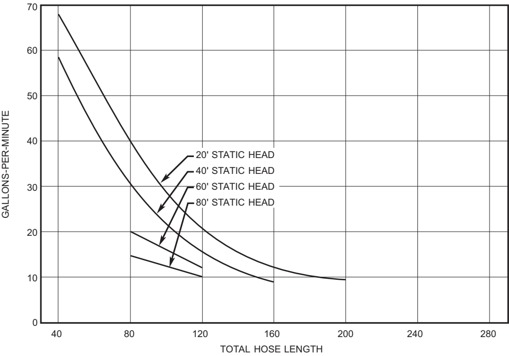
Figure H-14. CCN-150 Flow Rates - Cold #6 Fuel, 4" Hose.
