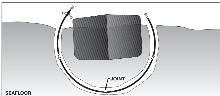
Figure 12-25B. Tunneling Lance Operations.
