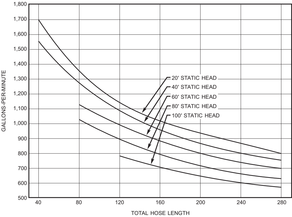
Figure H-10. CCN-150 Flow Rates - Water, 4" Hose.
