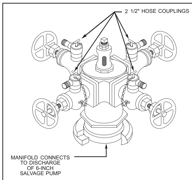
Figure 17-7. Firefighting Connection for Salvage Pumps.
