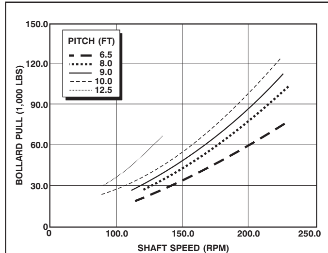
Figure G-2. Bollard Pull vs. Shaft Speed and Propeller Pitch for T-ATF-166 Class Ship Without Kort Nozzle.
