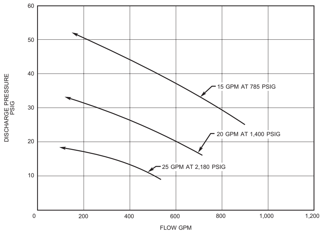
Figure H-9. 4-Inch Hydraulic Submersible Pump Performance Curves.
