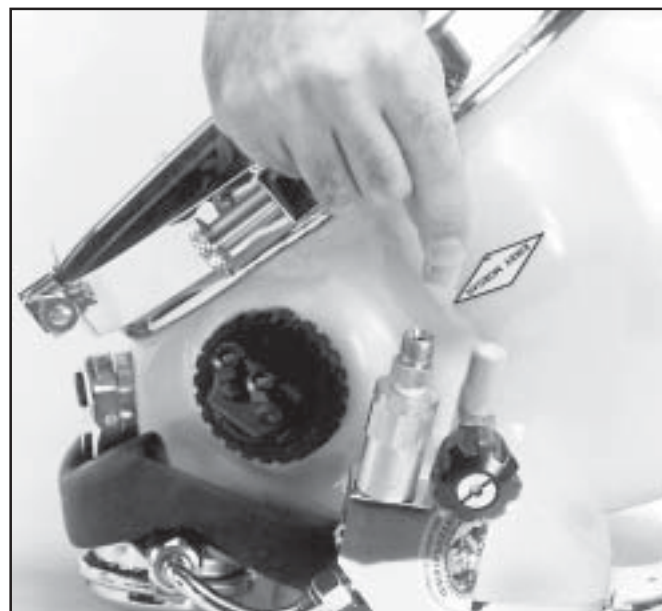
Cover the air inlet and auxiliary valve openings with dust caps when not in use.
