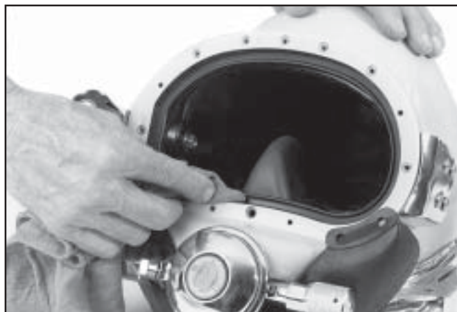
Clean the O-ring groove
